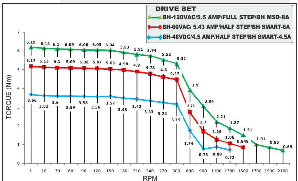
STEPPER MOTOR - BH86SH123-5504AKS-SZ
