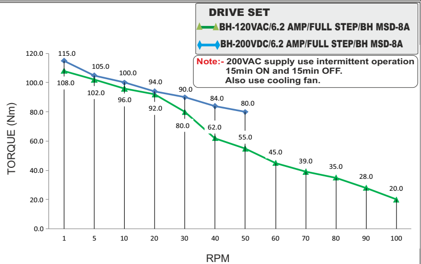
PLANETARY GEAR BOX STEPPER MOTOR - BH86SH156-6204PL-10
