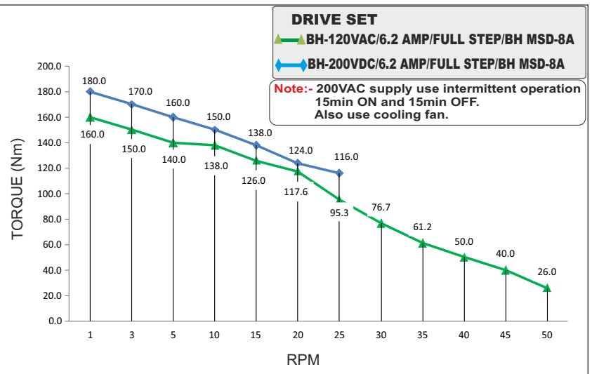
PLANETARY GEAR BOX STEPPER MOTOR - BH86SH156-6004PL-20
