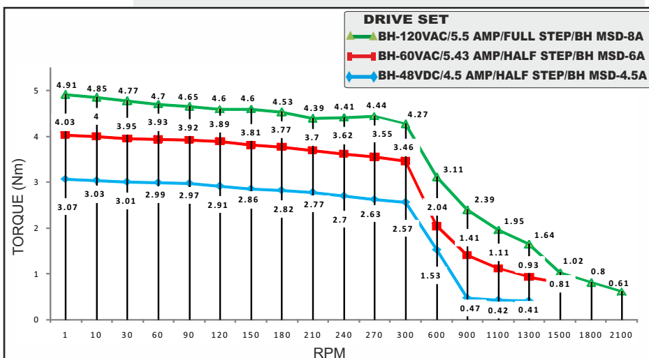
STEPPER MOTOR -BH86SH80-5504AKS-IP65
