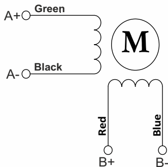
Wiring Diagram
