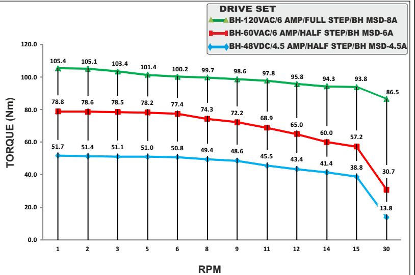
HELICAL WORM GEAR BOX STEPPER MOTOR - BH86SH118-6004HL-20
